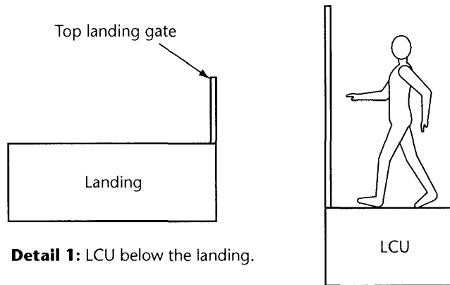
Figure E-3 Elaboration of Design Concept LCU – Landing Bridge
