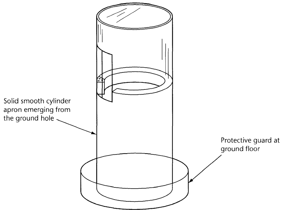
Figure E-2b View of Ground Guard and Raised LCU
