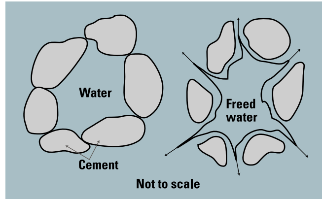
Figure 4-22. One mechanism by which water reducers work is dispersion: charged cement particles cling together, trapping water (left) and water reducers separate cement grains, releasing the water and making it available for hydration (right)
